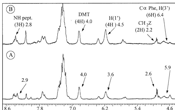
Figure 5. Part of the ^1\text{H} NMR spectra of the two chimeric PEG-conjugates in [\text{D}_6]\text{DMSO} : A) peptide first, B) oligonucleotide first
