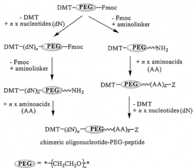
Scheme 1. General scheme showing the two alternative syntheses of a chimeric oligonucleotide-PEG-peptide on the same PEG-protected polymer
