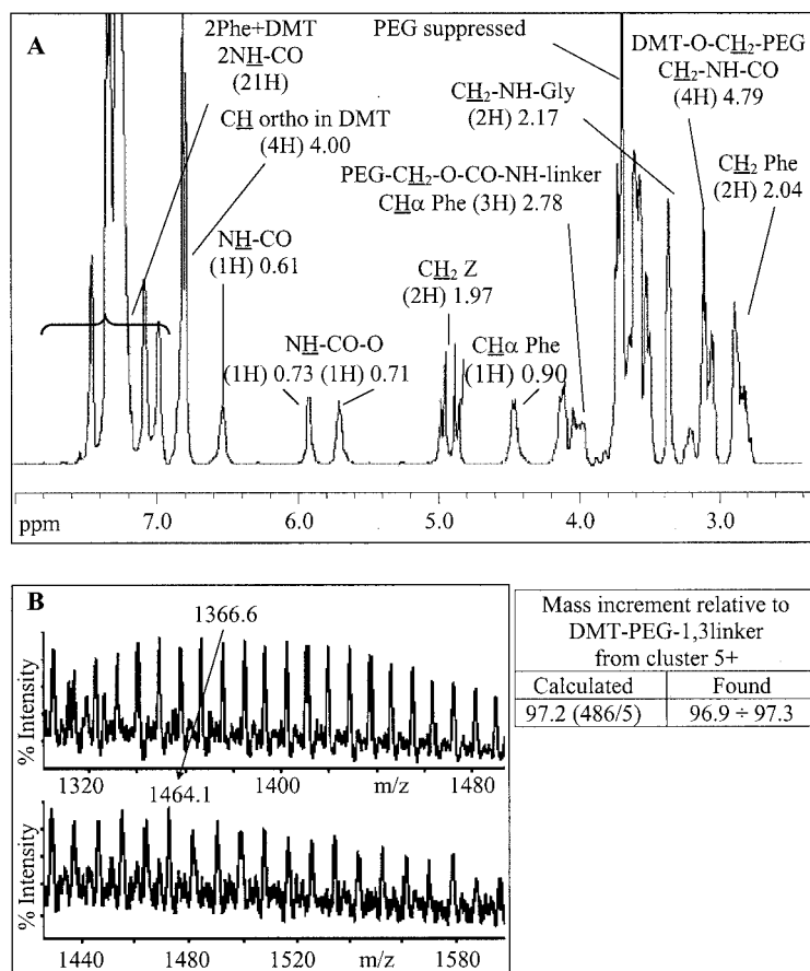
Figure 2. A) ^1\text{H} NMR spectrum of DMT-PEG-1,3-linker-Gly-L-Phe-D-Phe-Z in \text{CDCl}_3 ; B) part of the ESI spectrum
