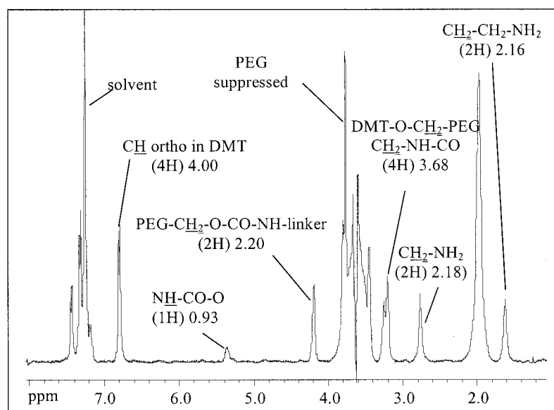
Figure 1. 1 H NMR spectrum of DMT-PEG-1,3-diaminopropane in CDCl 3
