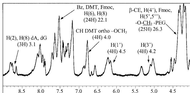
Figure 3. Partial ^1\text{H} NMR spectrum of DMT-d(CGAT)-PEG-Fmoc in [\text{D}_6]\text{DMSO}
