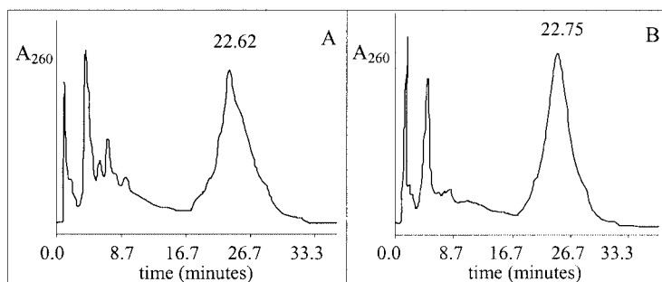
Figure 4. Ion-exchange HPLC of the two chimeric PEG-conjugates: A) peptide first, B) oligonucleotide first
